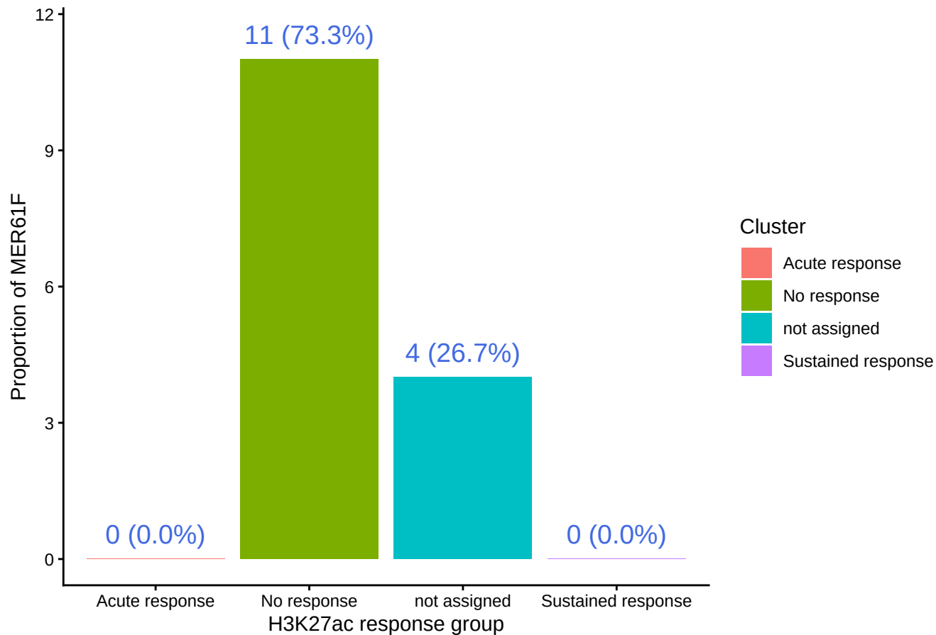
Proportion of MER61F across each H3K27ac set
